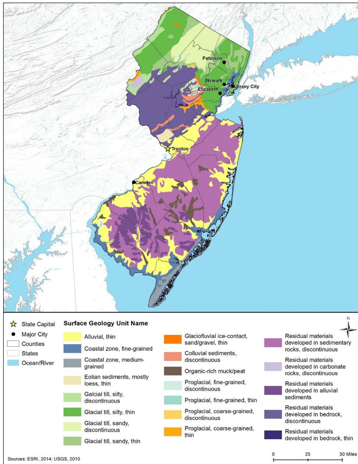
Figure 10.1.3-2: Generalized Surface Geology for New Jersey
